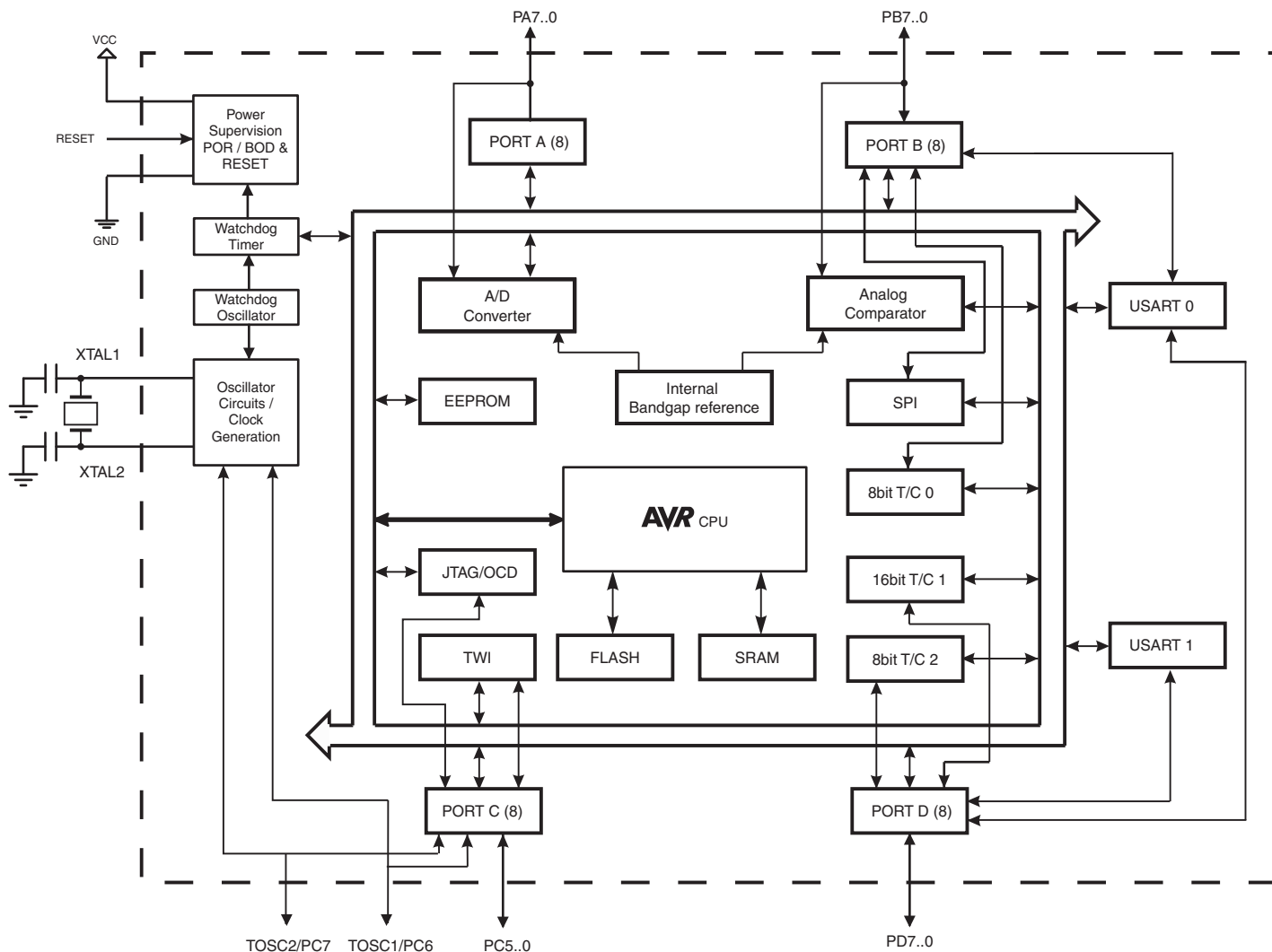
Figure 2-1. Block Diagram
