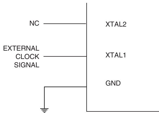
Figure 3. External Clock Drive Configuration
