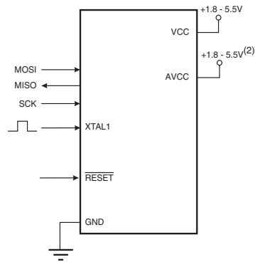
Figure 24-10. Serial Programming and Verify (1)
