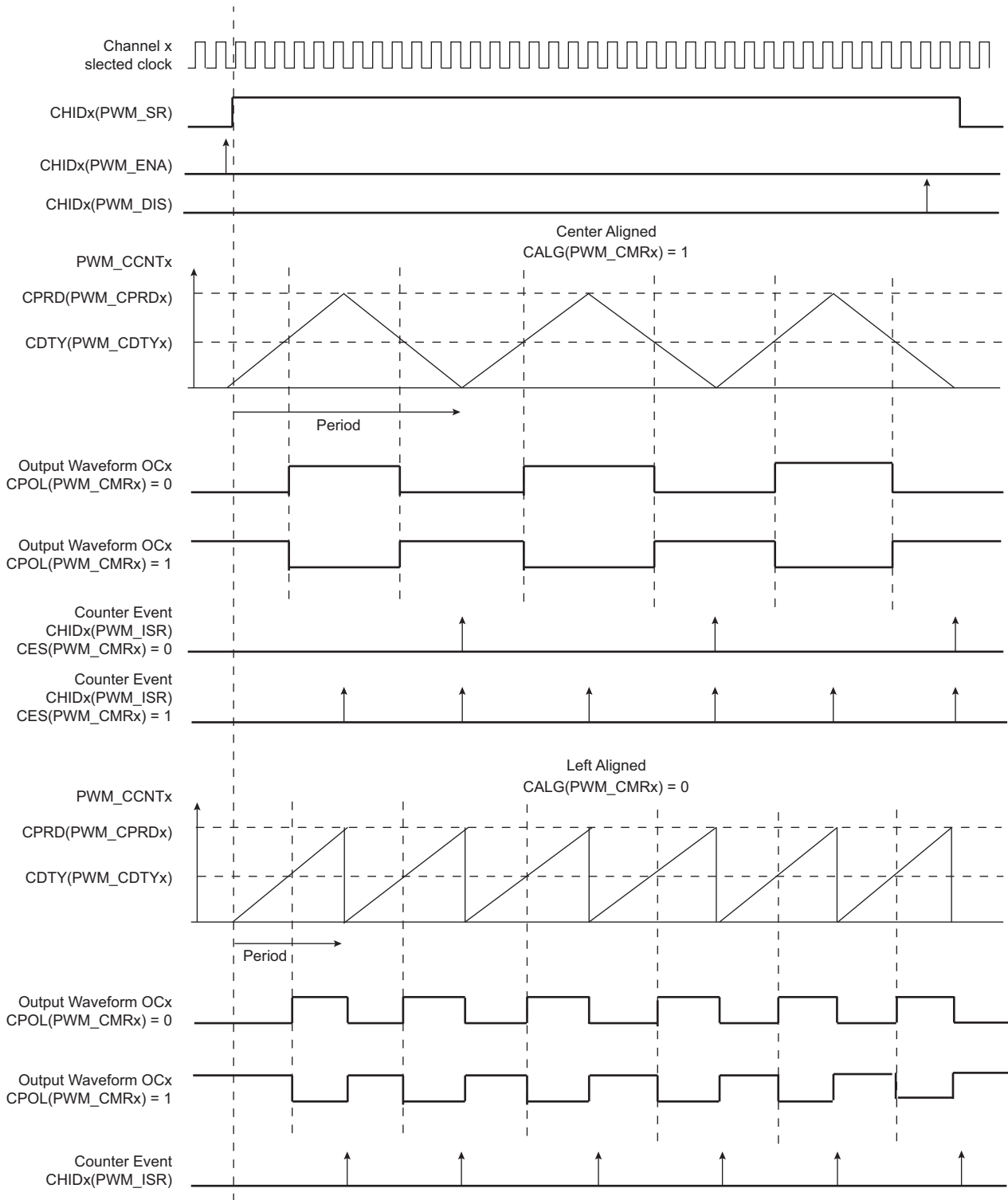
Figure 46-5. Waveform Properties
