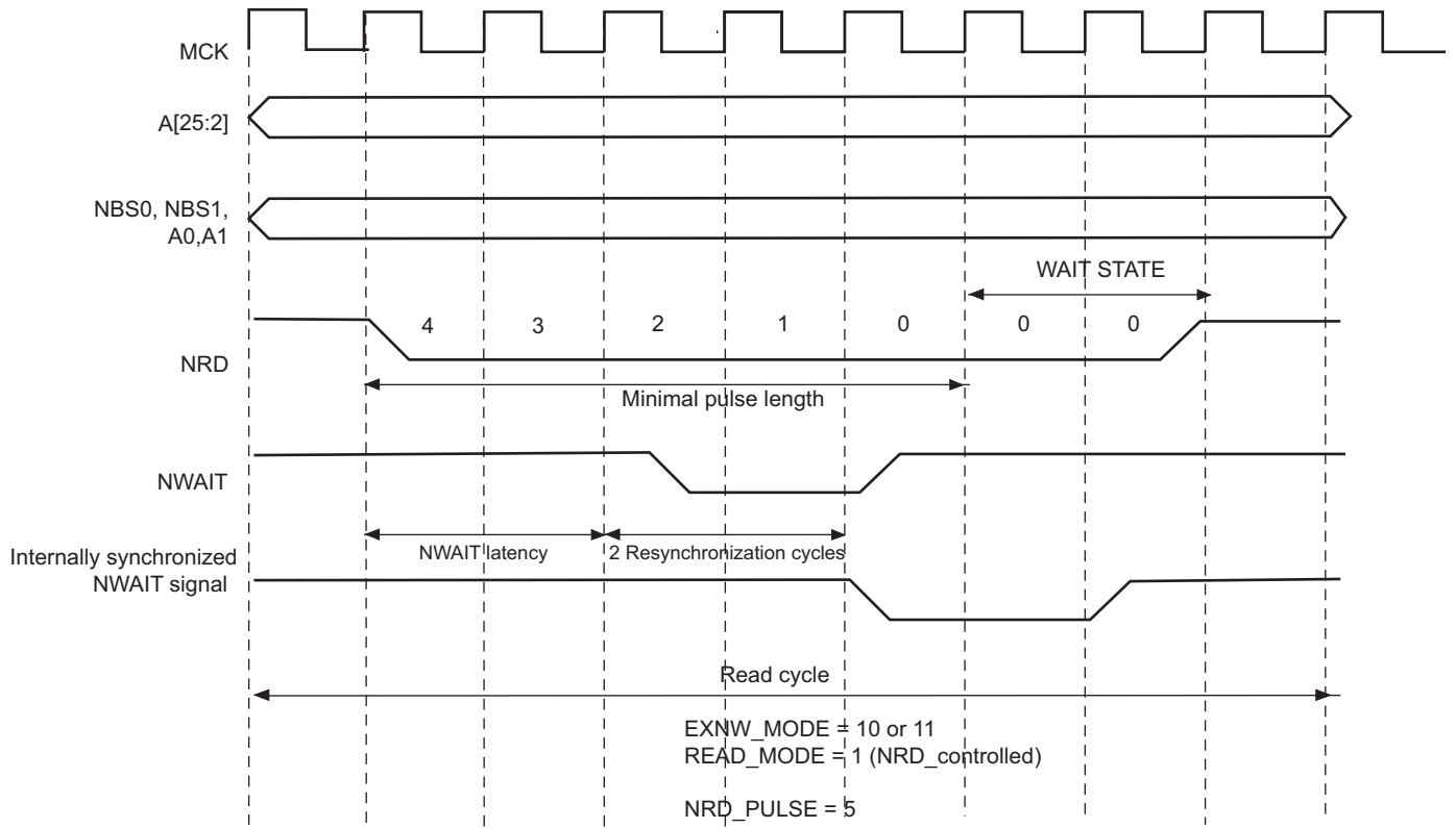
Figure 29-27. NWAIT Latency
