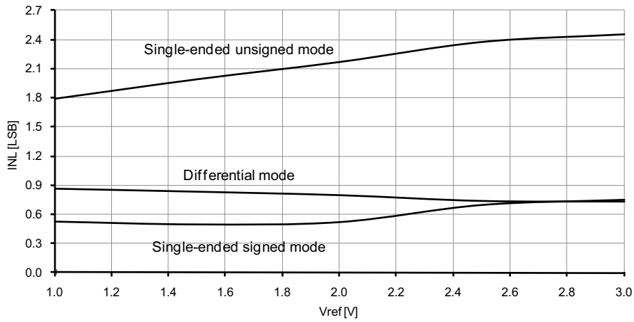
Figure 37-204. INL error vs. external V_{\text{REF}} . T = 25^\circ\text{C} , V_{CC} = 3.6\text{V} , external reference.
