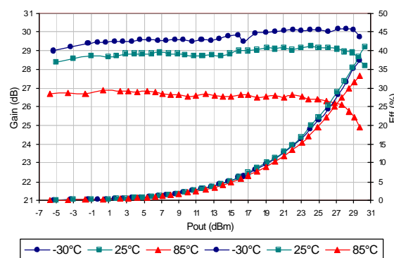
Figure 28 IS-98D Gain & Eff. versus Pout @ 836.5 MHz Vcc: 4.2V, Vref: 3.0V, Vmode: 0.0V
