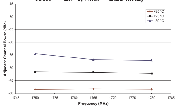
Figure 12: Adjacent Channel Power vs. Freq. ( P_{OUT} = +16.0 dBm, V_{CC} = +3.5 V, V_{REF} = +3.0 V, V_{MODE} = +2.7 V, \Delta f_{ACP} = 2.25 MHz)
