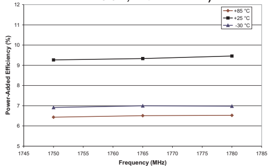
Figure 14: Power-Added Efficiency vs. Freq. ( P_{OUT} = +16.0 dBm, V_{CC} = +3.5 V, V_{REF} = +3.0 V, V_{MODE} = +2.7 V)
