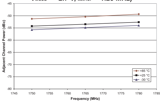
Figure 9: Adjacent Channel Power vs. Freq. ( P_{OUT} = +28.5 dBm, V_{CC} = +3.5 V, V_{REF} = +3.0 V, V_{MODE} = +2.7 V, \Delta f_{ACP} = 1.25 MHz)
