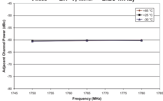
Figure 11: Adjacent Channel Power vs. Freq. ( P_{OUT} = +28.5 dBm, V_{CC} = +3.5 V, V_{REF} = +3.0 V, V_{MODE} = +2.7 V, \Delta f_{ACP} = 2.25 MHz)
