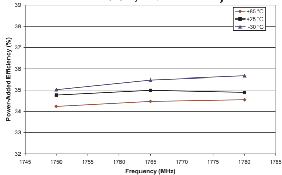
Figure 13: Power-Added Efficiency vs. Freq. ( P_{OUT} = +28.5 dBm, V_{CC} = +3.5 V, V_{REF} = +3.0 V, V_{MODE} = +2.7 V)
