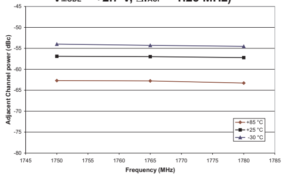
Figure 10: Adjacent Channel Power vs. Freq. ( P_{OUT} = +16.0 dBm, V_{CC} = +3.5 V, V_{REF} = +3.0 V, V_{MODE} = +2.7 V, \Delta f_{ACP} = 1.25 MHz)
