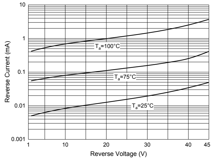
Fig. 2 - Reverse Characteristics
