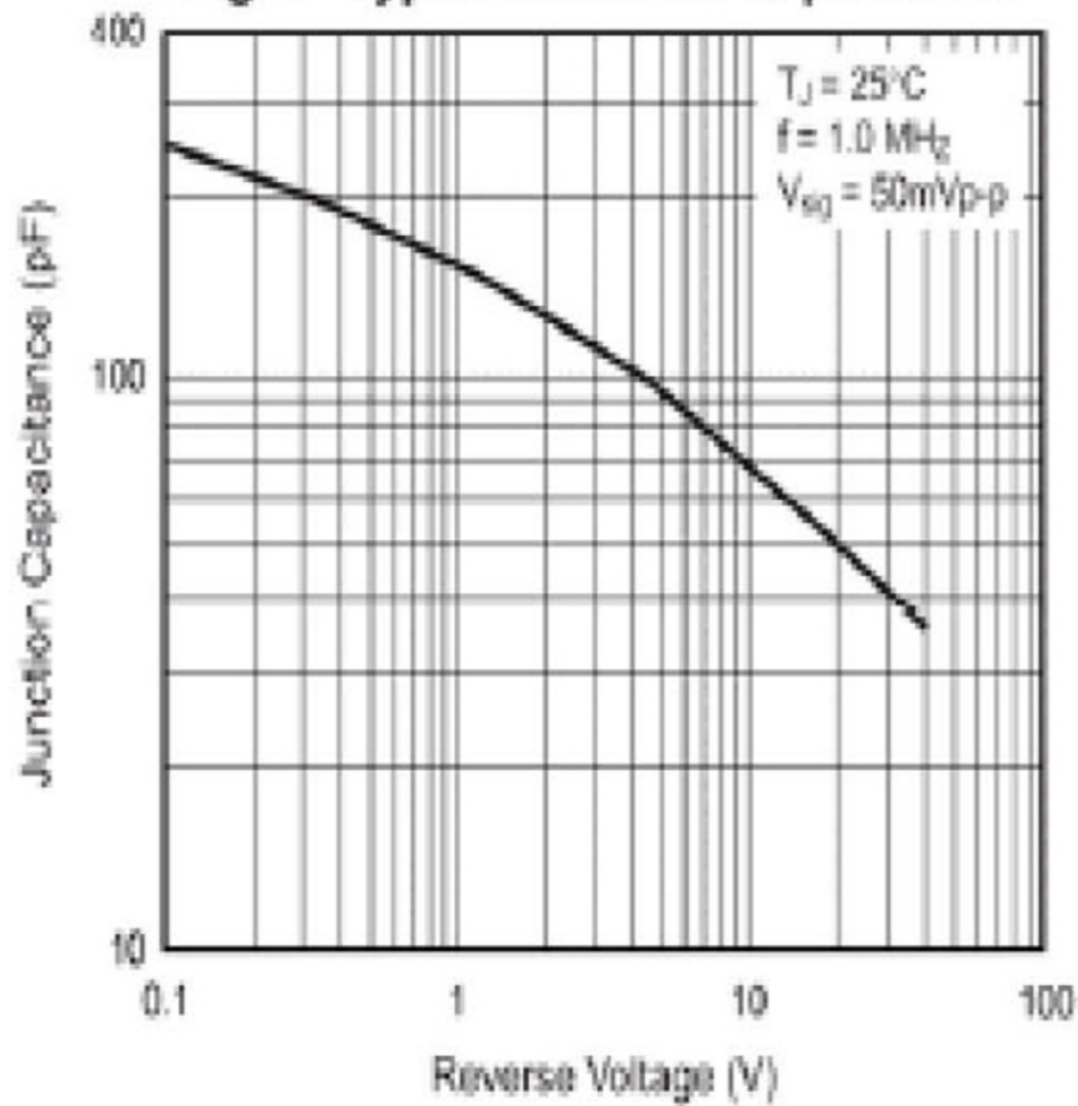
Fig. 5 - Typical Junction Capacitance
