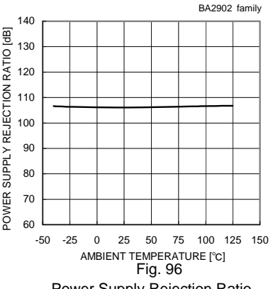
Power Supply Rejection Ratio - Ambient Temperature
