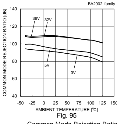
Common Mode Rejection Ratio - Ambient Temperature
