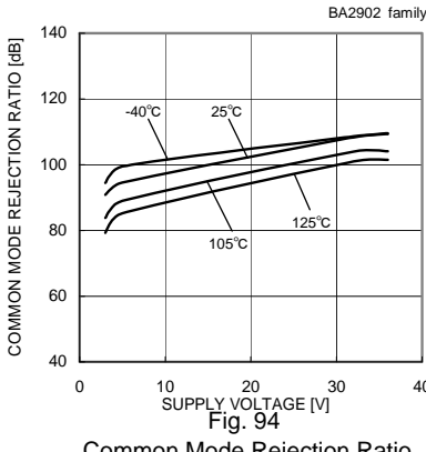
Common Mode Rejection Ratio - Supply Voltage
