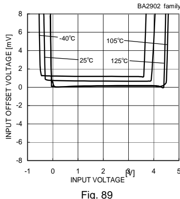
Input Offset Voltage - Common Mode Input Voltage (VCC=5[V])
