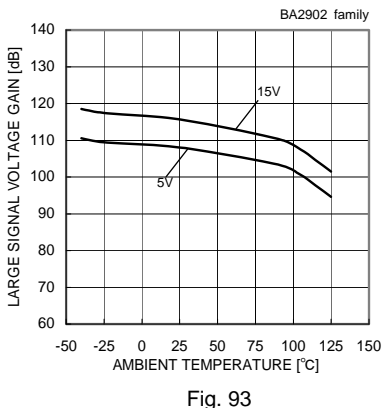
Large Signal Voltage Gain - Ambient Temperature (RL=2[kΩ])
