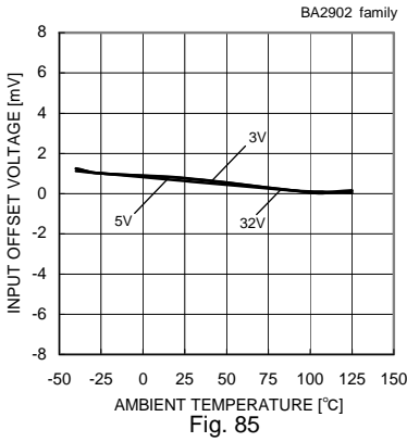
Input Offset Voltage - Ambient Temperature (Vicm=0[V], VOUT=1.4[V])
