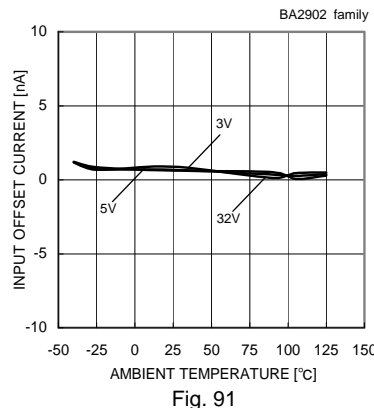
Input Offset Current - Ambient Temperature (Vicm=0[V], VOUT=1.4[V])
