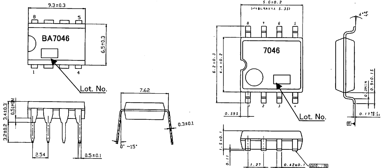
DIP8 (Unit : mm)
