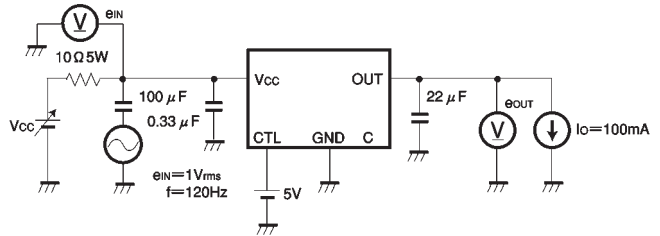
Fig.2 Measurement circuit for ripple rejection ratio
