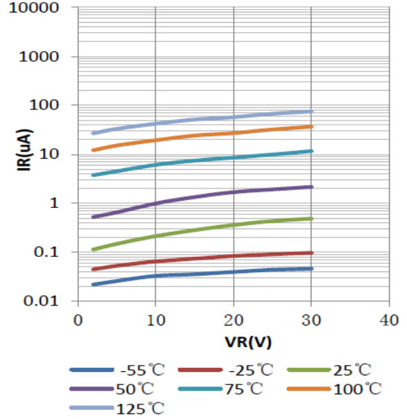
Figure 2. Reverse Characteristics
