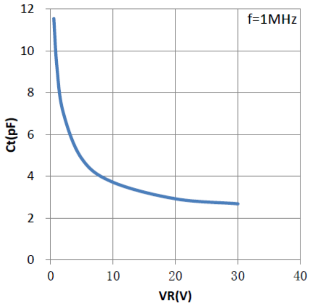
Figure 3. Capacitance
