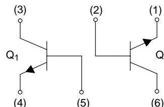
BC847CDXV6T1
