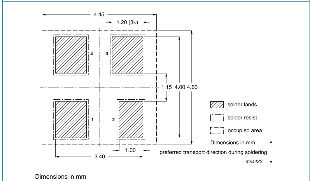
Dimensions in mm Fig 12. Reflow soldering footprint SOT143B
