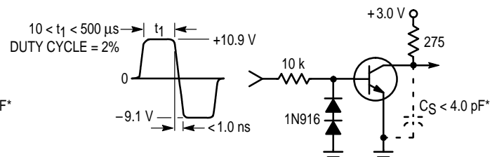
Figure 2. Turn–Off Time
