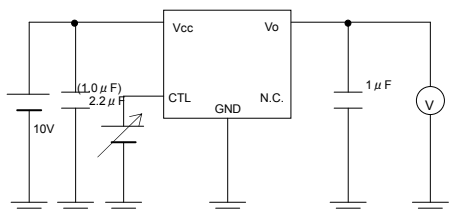
Measurement Circuit of Fig.11 and Fig.23
