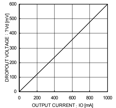
Fig.18 Dropout Voltage (Vcc=Vo × 0.95V) (Io=0mA→1000mA)
