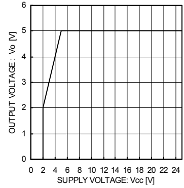
Fig.15 Line Regulation (Io=0mA)
