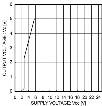
Fig.16 Line Regulation (Io=500mA)
