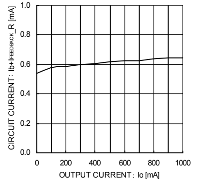
Fig.21 Circuit Current (Io=0mA→1000 mA)
