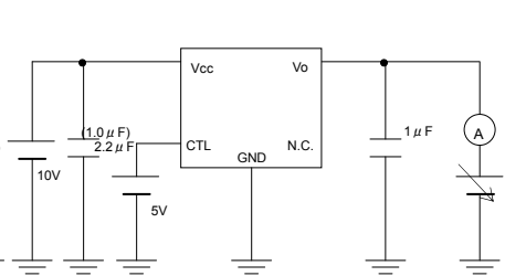
Measurement Circuit of Fig.5 and Fig.17
