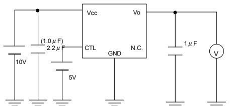
Measurement Circuit of Fig.8 and Fig.20
