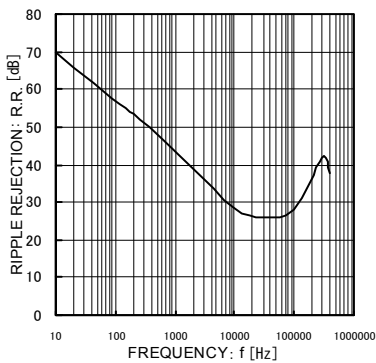
Fig.19 Ripple Rejection (Io=100mA)
