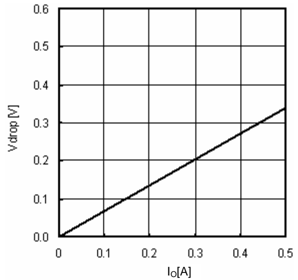
Fig.22 Minimum dropout Voltage 2 ( V_{CC}=2.4V , T_a=25^{\circ}C )
