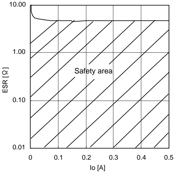
Fig.19 ESR Condencer
