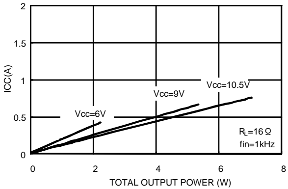
Fig. 20 Current Consumption - Output Power
