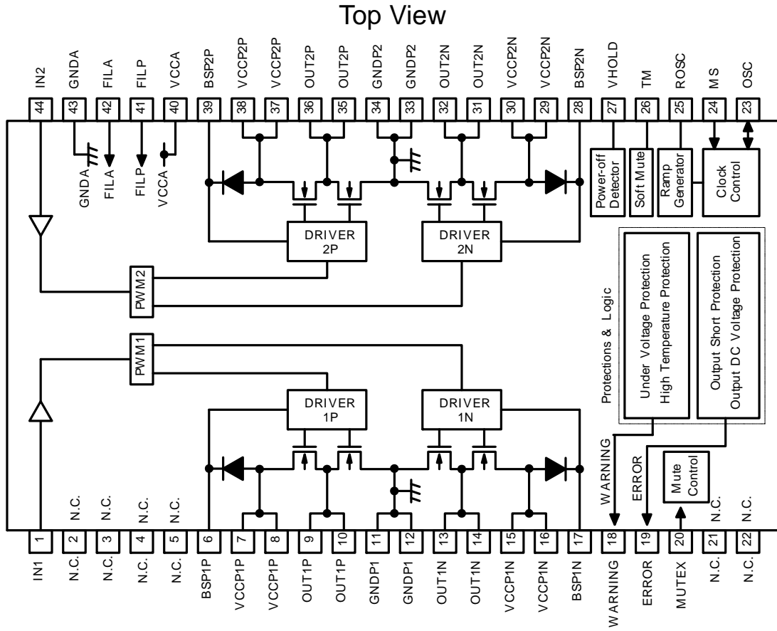
Fig. 22 Pin Assignment Diagram
