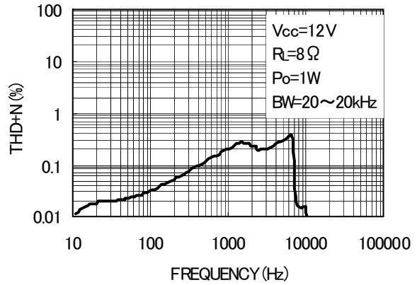
Fig. 2 THD+N - Frequency
