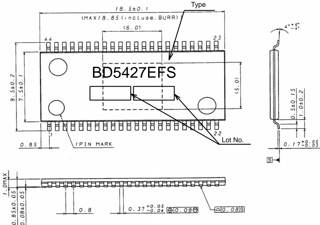
Fig. 23 Outer Dimensions and Incriptions of HTSSOP-A44 Package
