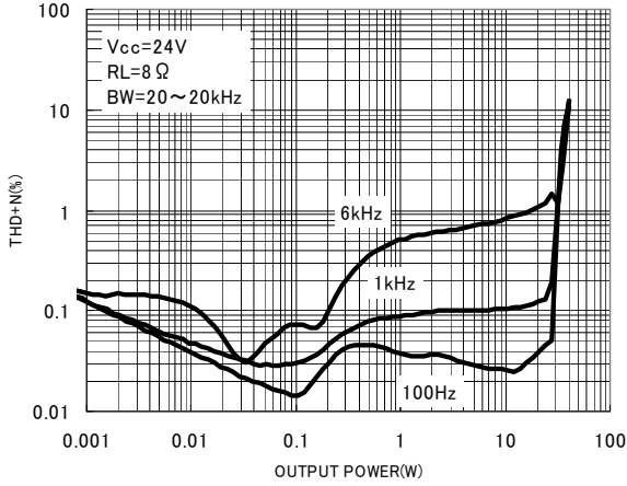
Fig.22 Output power—THD+n
