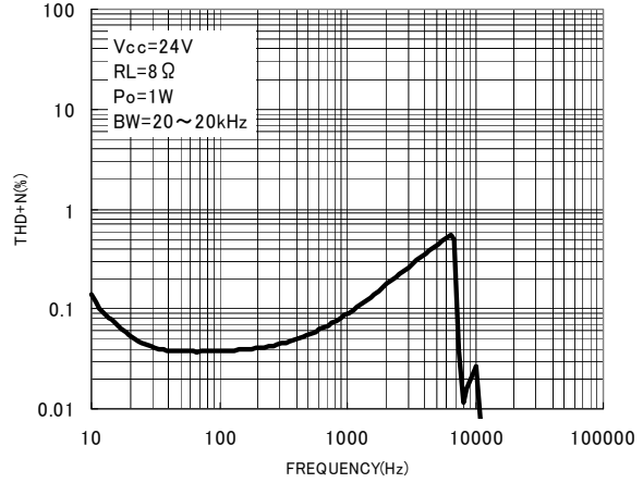
Fig.23 Frequency—THD+n
