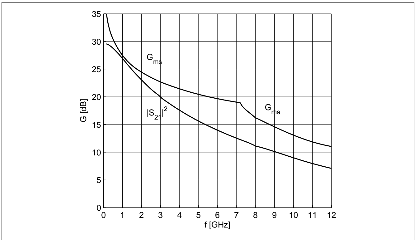
Figure 7-12 Gain G_{ma}, G_{ms}, |S_{21}|^2 = f(f), V_{CE} = 3 \text{ V}, I_C = 15 \text{ mA}
