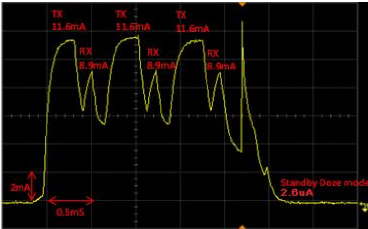
Figure 3: Typical peak current consumption profile (with DCDC ON) during advertising in slave mode @ TX PWR +4dBm. UART is OFF. Last spike is DCDC being turned off.
