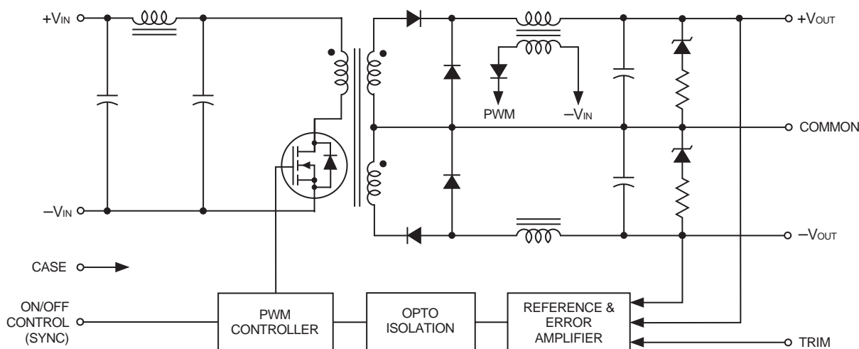
Figure 1. Simplified Schematic
