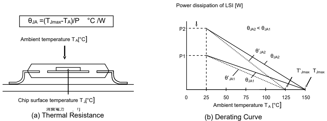
Figure 13. Thermal resistance and derating curve
