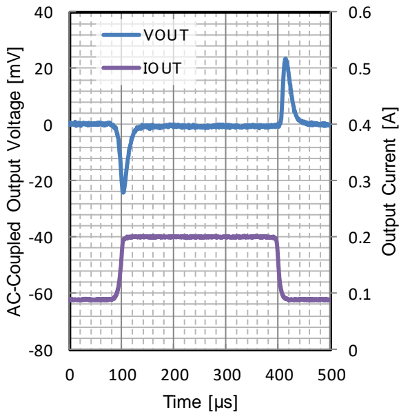
Figure 196. Load Transient V_{OUT} = 3.0\text{ V} t_R = t_F = 10\text{ }\mu\text{s} , I_{OUT} = 90\text{ mA to }210\text{ mA} , C_{OUT} = 10\text{ }\mu\text{F} T_j = 150\text{ }^\circ\text{C}
