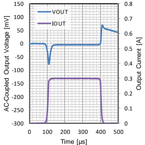
Figure 149. Load Transient
