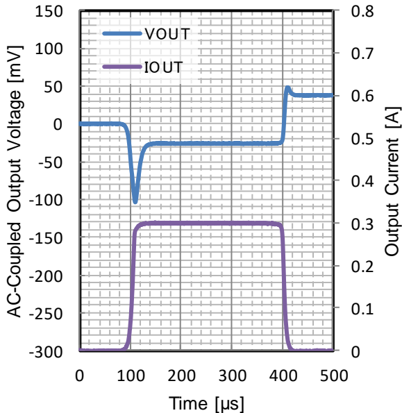
Figure 148. Load Transient
