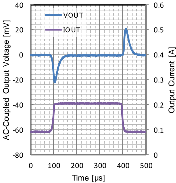
Figure 194. Load Transient V_{OUT} = 3.0\text{ V} t_R = t_F = 10\text{ }\mu\text{s} , I_{OUT} = 90\text{ mA to }210\text{ mA} , C_{OUT} = 10\text{ }\mu\text{F} T_j = -40\text{ }^\circ\text{C}
