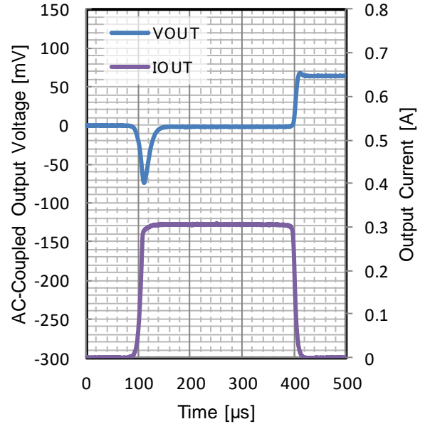
Figure 147. Load Transient
