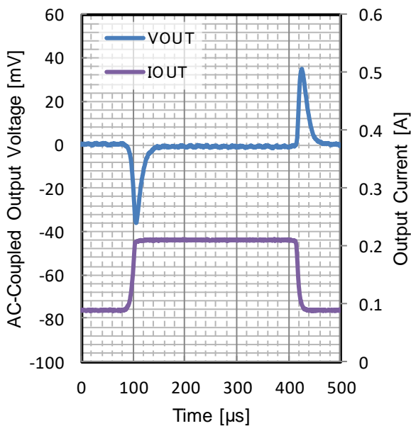
Figure 237. Load Transient V_{OUT} = 3.3\text{ V}
