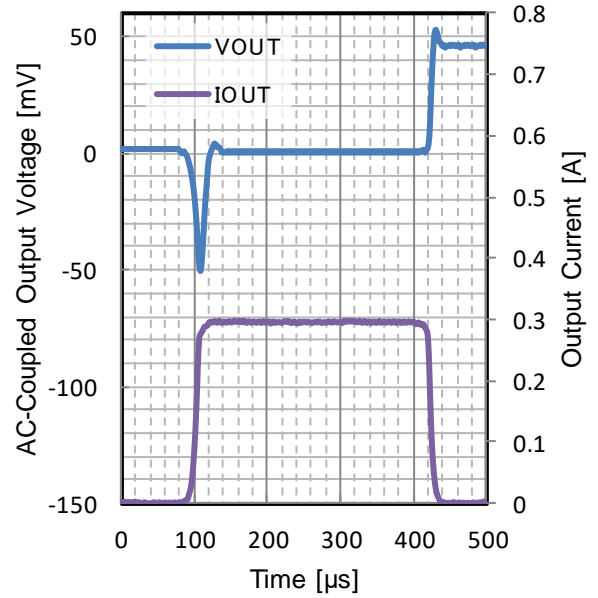
Figure 62. Load Transient
