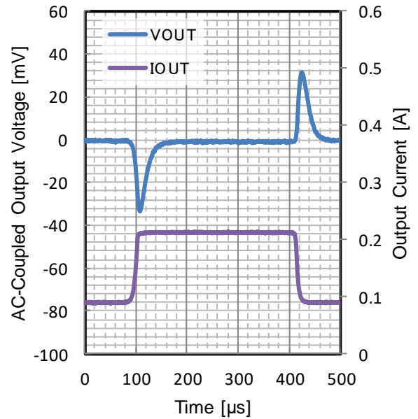
Figure 236. Load Transient V_{OUT} = 3.3\text{ V}
