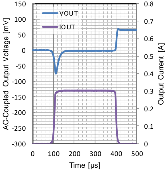
Figure 146. Load Transient
