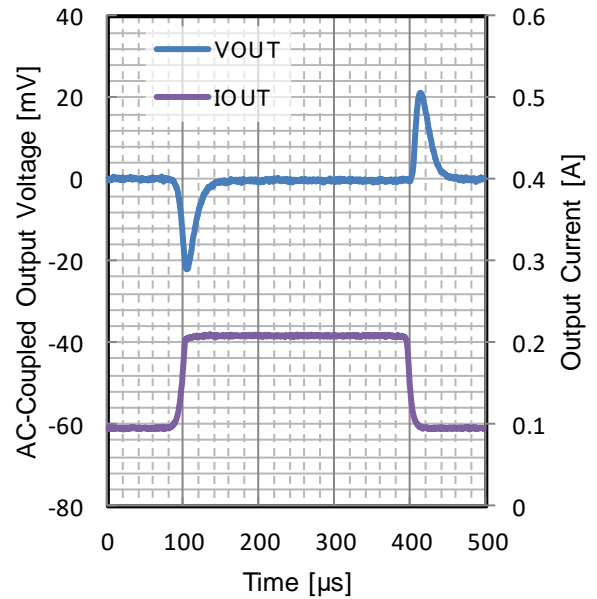
Figure 195. Load Transient V_{OUT} = 3.0\text{ V} t_R = t_F = 10\text{ }\mu\text{s} , I_{OUT} = 90\text{ mA to }210\text{ mA} , C_{OUT} = 10\text{ }\mu\text{F} T_j = 25\text{ }^\circ\text{C}
