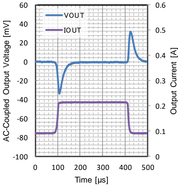
Figure 235. Load Transient V_{OUT} = 3.3\text{ V}
