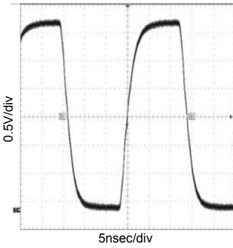
Fig.16 36MHz output waveform (CL=15pF, Ta=25 °C)
