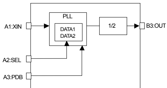
Fig.54 Block diagram
