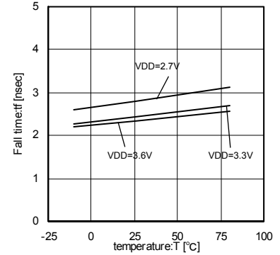
Fig.36 36MHz Temperature - Fall-time
