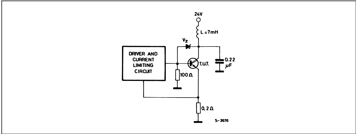
Figure 12: Functional Test Circuit
