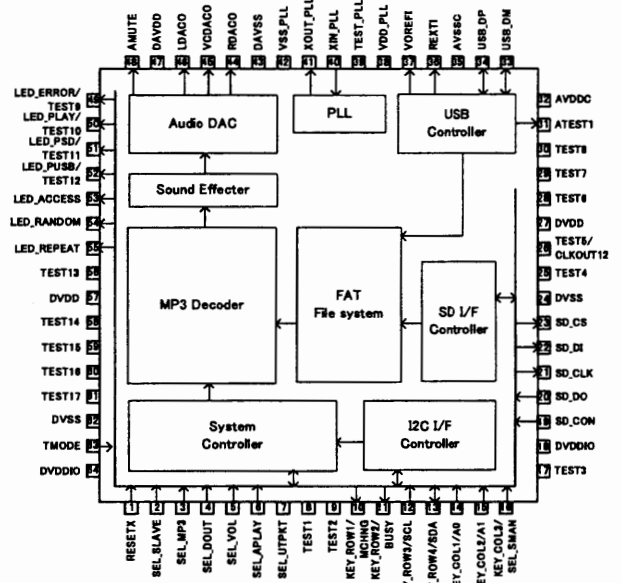
Figure 2. Block diagram
