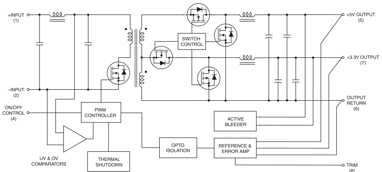
Figure 1. Simplified Schematic
