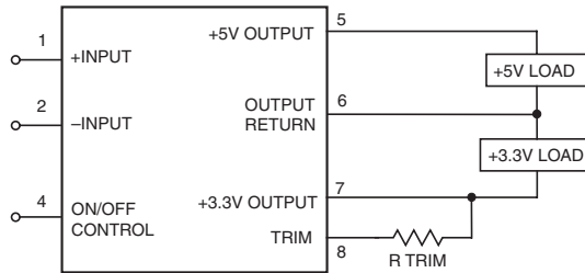
Figure 4. Decrease Output Voltage Trim Connections Using A Fixed Resistor
