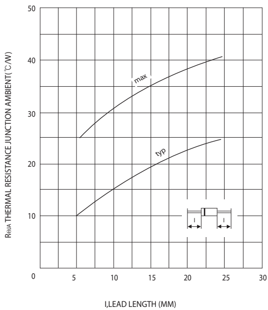
FIG.3-TYPICAL THERMAL IMPEDANCE
