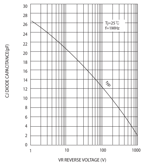
FIG.4-TYPICAL JUNCTION CAPACITANCE
