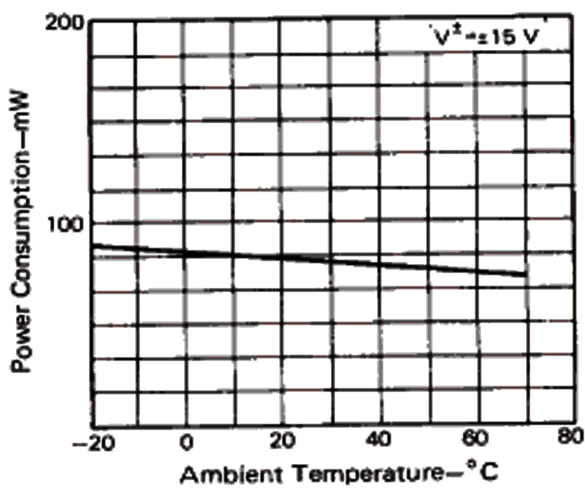
POWER CONSUMPTION
