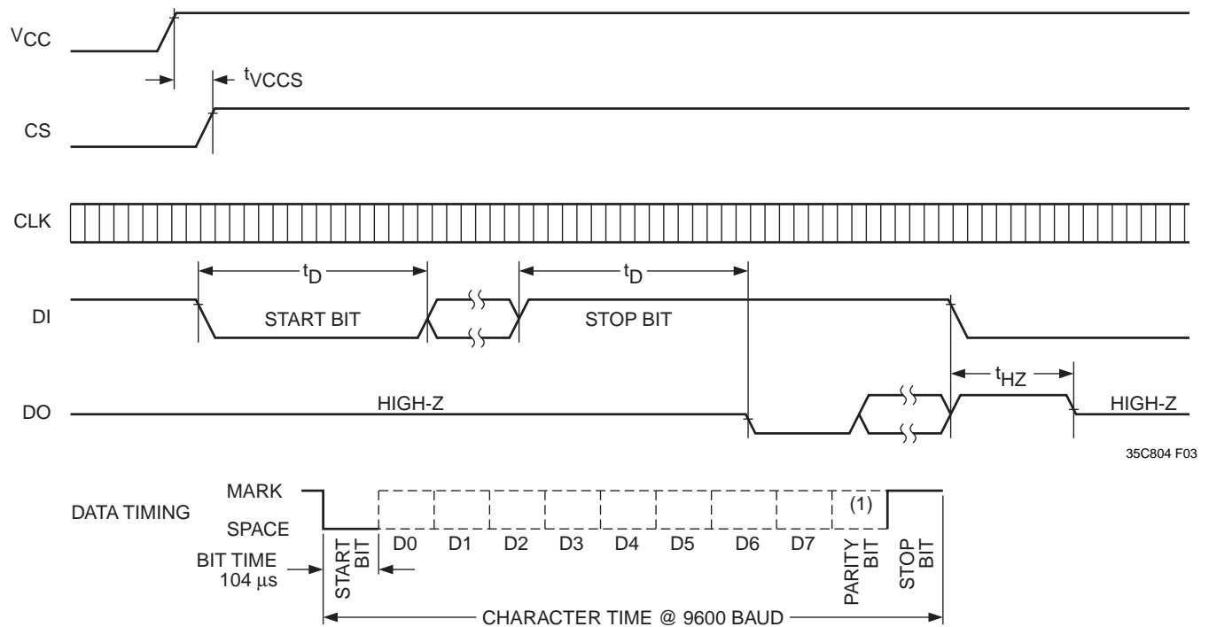
Figure 1. A.C. Timing
