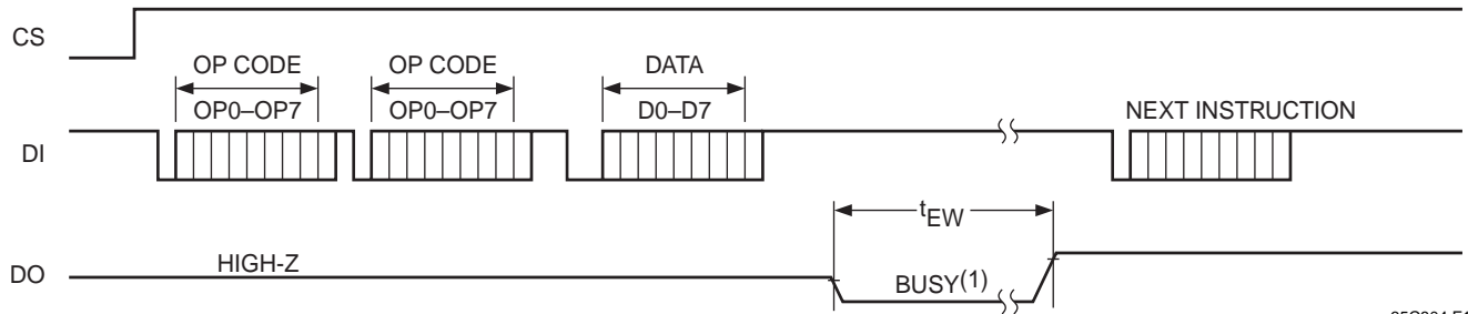
Figure 16. WRAL Timing (x8 Format)
