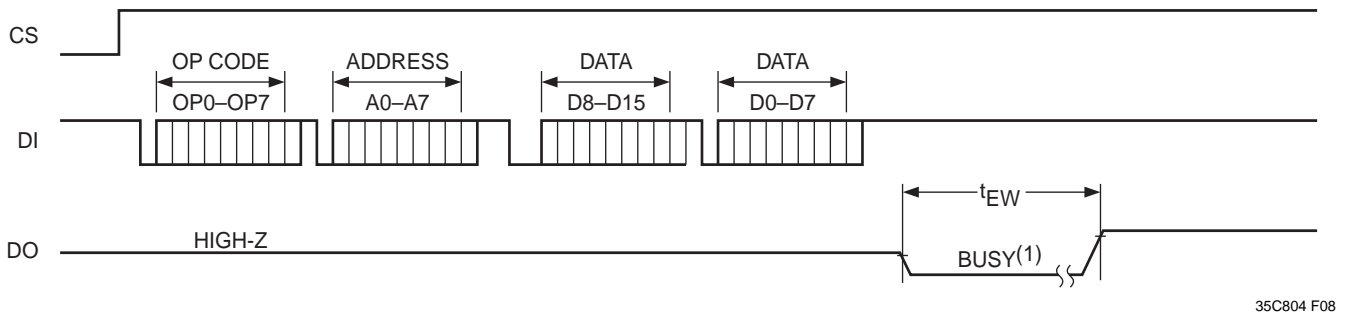
Figure 5. Program/Erase Timing (x16 Format)
