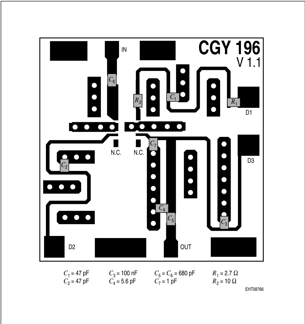
Figure 9 Test Board Layout (900 MHz ISM - Application)
