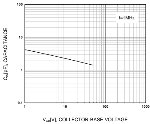
fig5.Collector Output Capacitance
