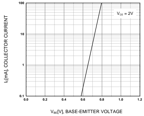
fig4.Base-Emitter On Voltage
