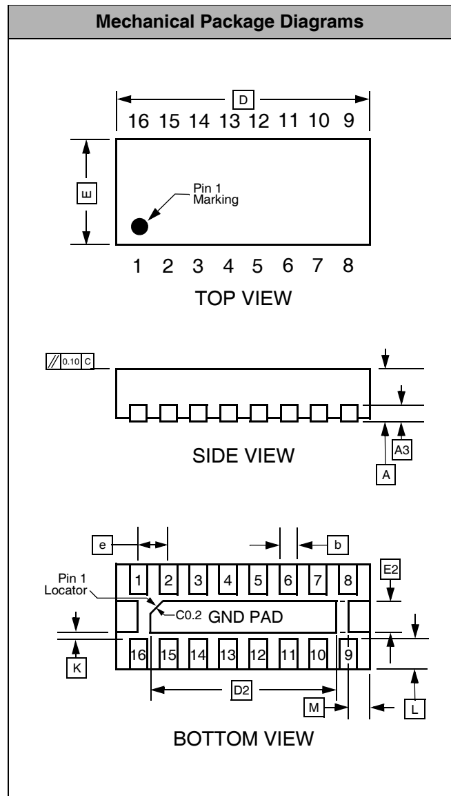
Dimensions for 16-Lead, 0.5mm pitch TDFN package
