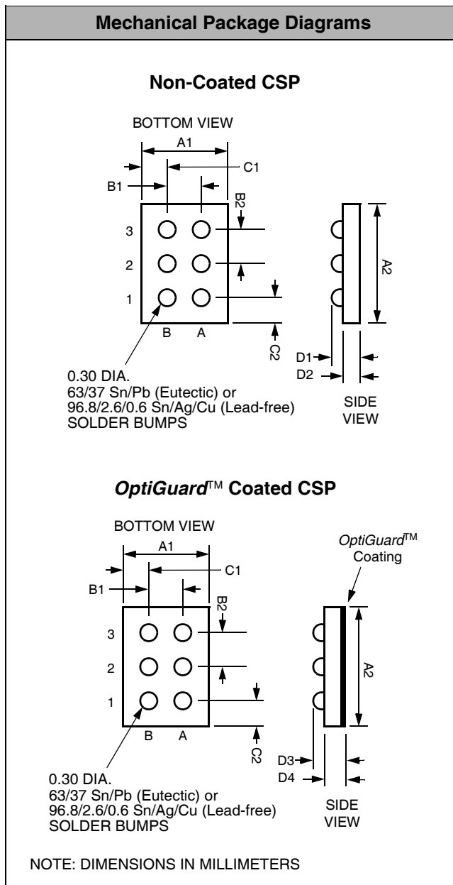
Package Dimensions for CM1418-0xCS/CP 6-bump Chip Scale Package
