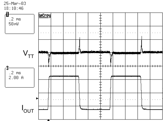
VTT Transient Response
