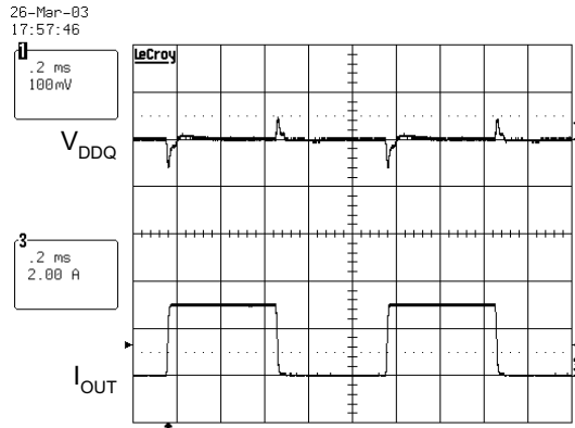
VDDQ Transient Response
