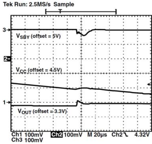
Figure 18. V_{CC} Power Down ( V_{SBY} = 5V , Load = 300 mA)
