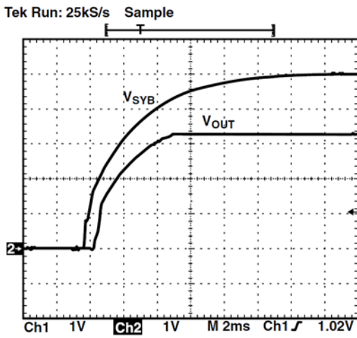
Figure 13. V_{SBY} Cold Start (Load = 400 mA)
