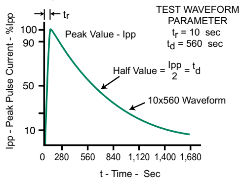
10x560 \mu S PULSE WAVE FORM
