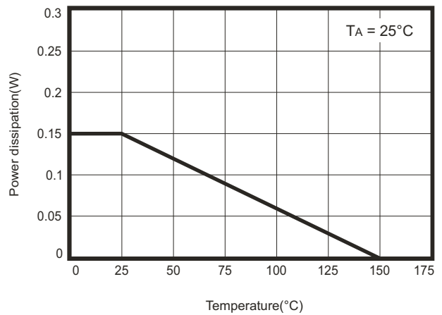
Fig.4 Steady state power derating
