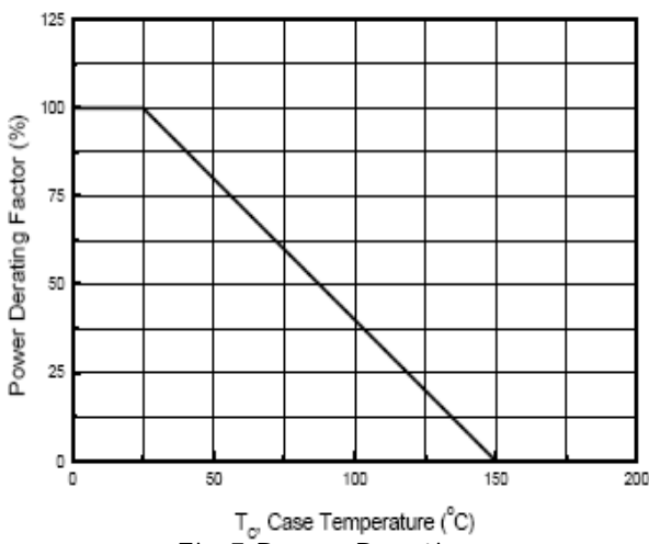
Fig. 5 Power Derating
