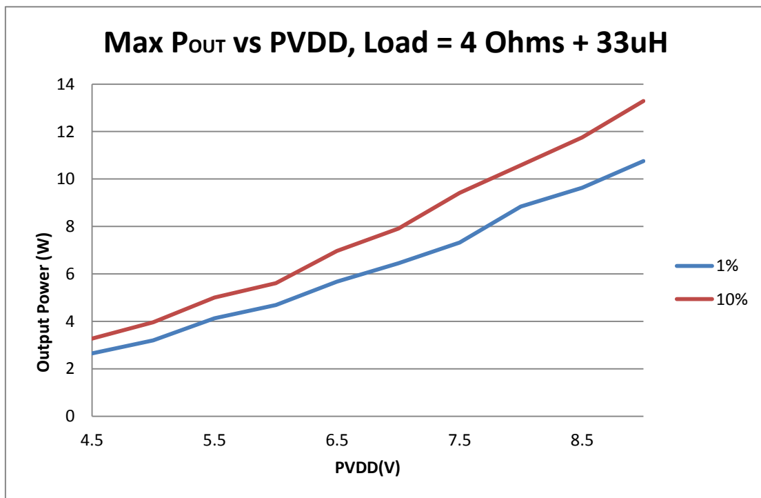
Figure 12: Maximum output power (P out ) versus supply voltage (4 Ω + 33 μH)
