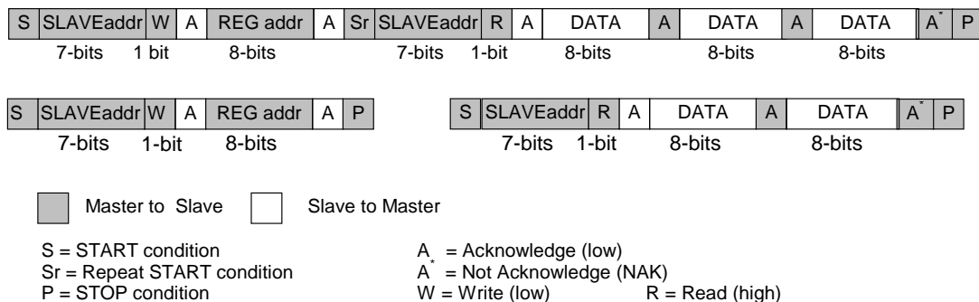
Figure 36: Examples of I 2 C Page Read (SDA line)
