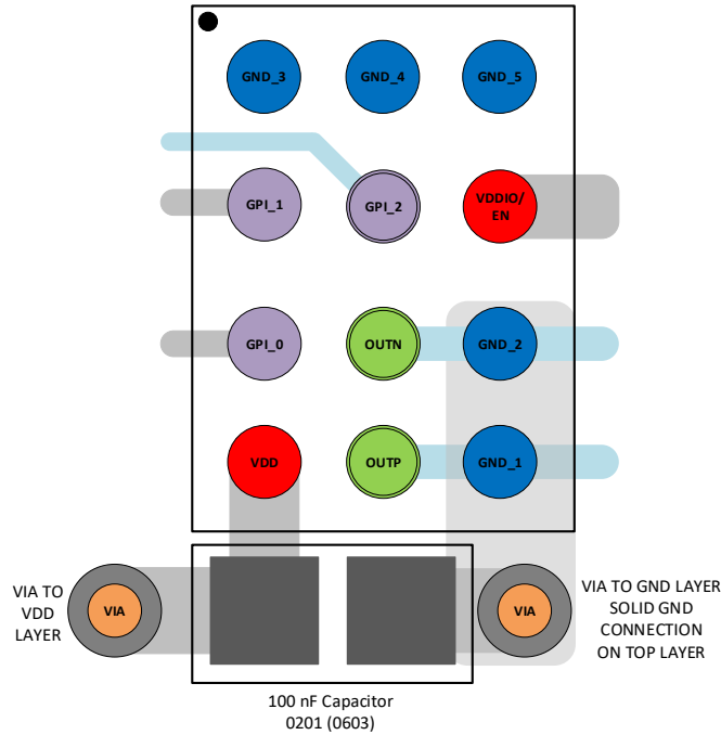
Figure 15: WLCSP Example PCB Layout
