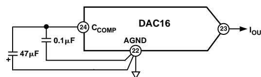
Figure 21b. Recommended Compensation Scheme to AGND
