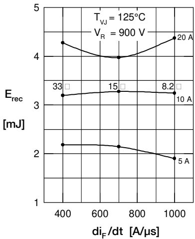
Fig. 5 Typ. recovery energy E_{rec} versus di/dt
