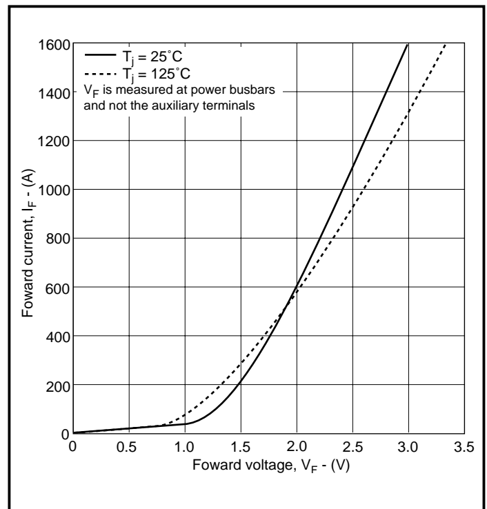
Fig. 6 Diode typical forward characteristics
