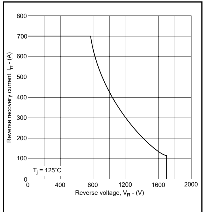
Fig. 8 Diode reverse bias safe operating area
