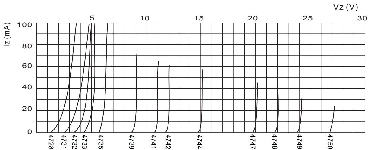
FIG.1 – BREAKDOWN CHARACTERISTICS
