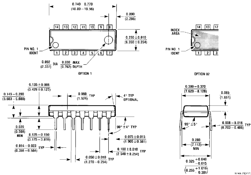
14-Lead Molded Dual-In-Line Package (N) Order Number DM74S140N Package Number N14A
