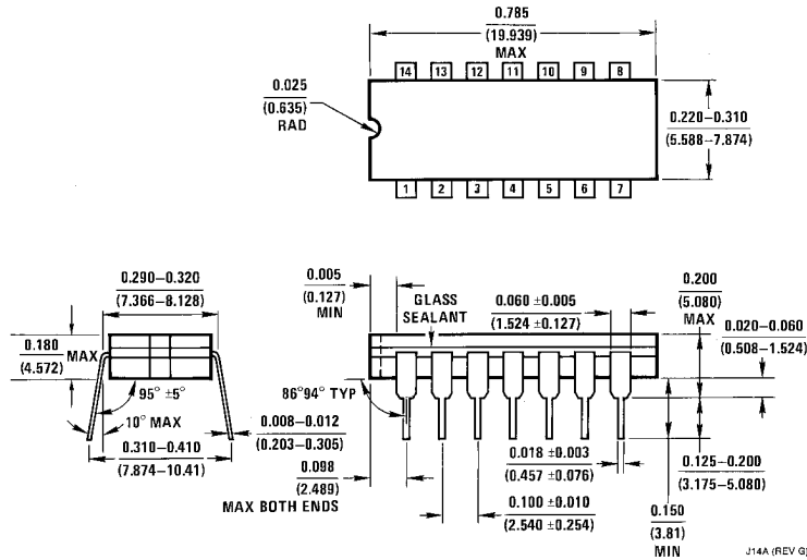
14-Lead Ceramic Dual-In-Line Package (J) Order Number DM54S140J Package Number J14A
